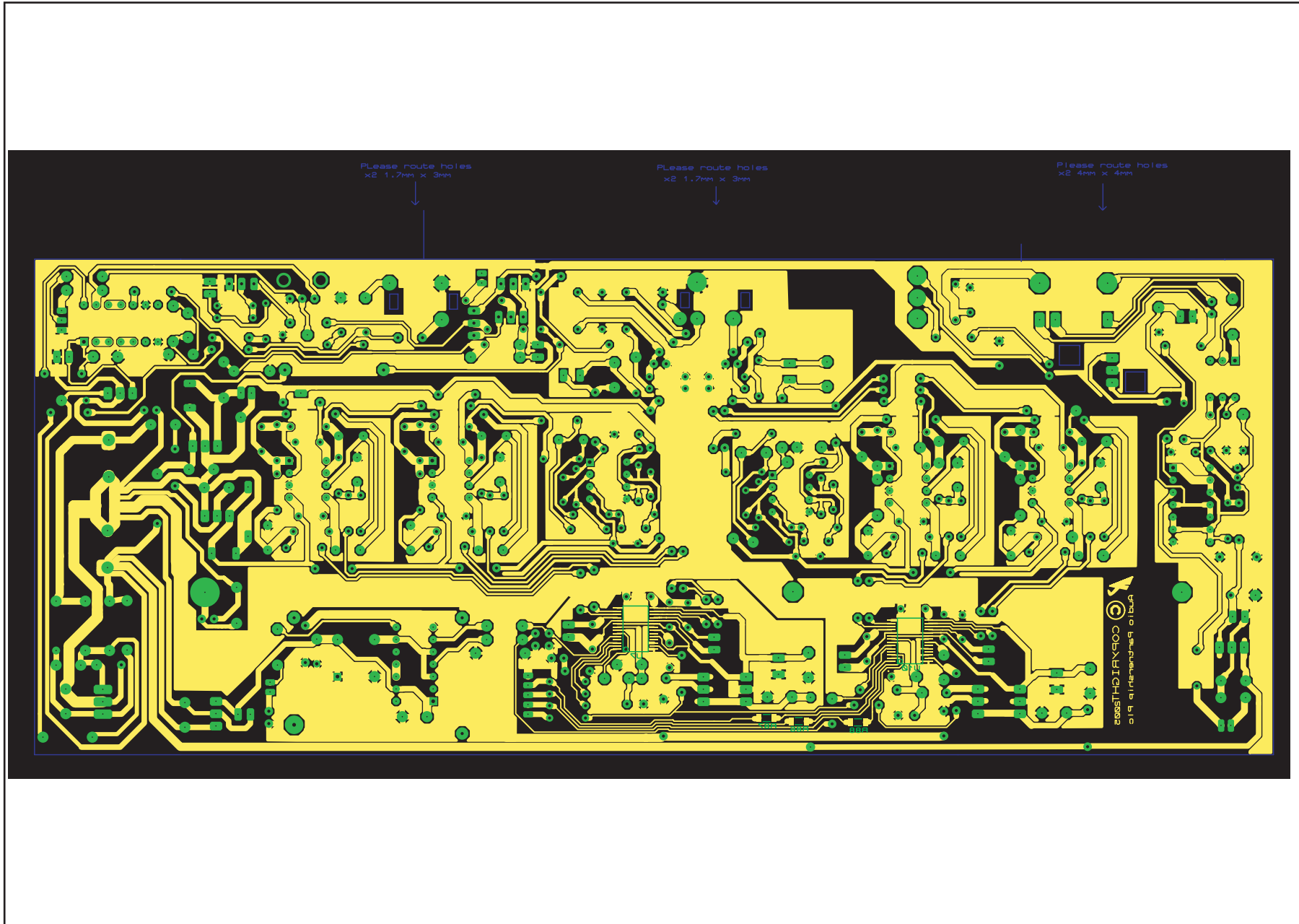
API7613/6 DAC Board PCB Layout (Bottom Side)
