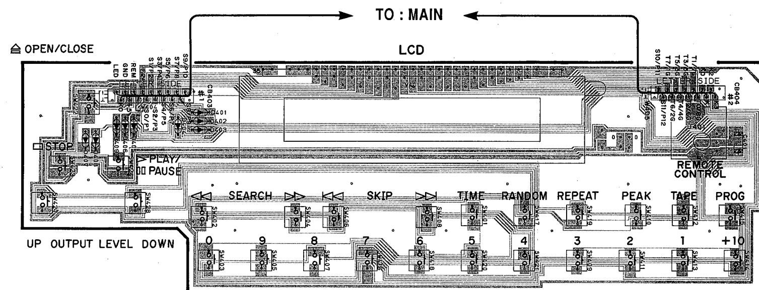
CDX - 570 OPERATION P. C. B. ( 2 )
