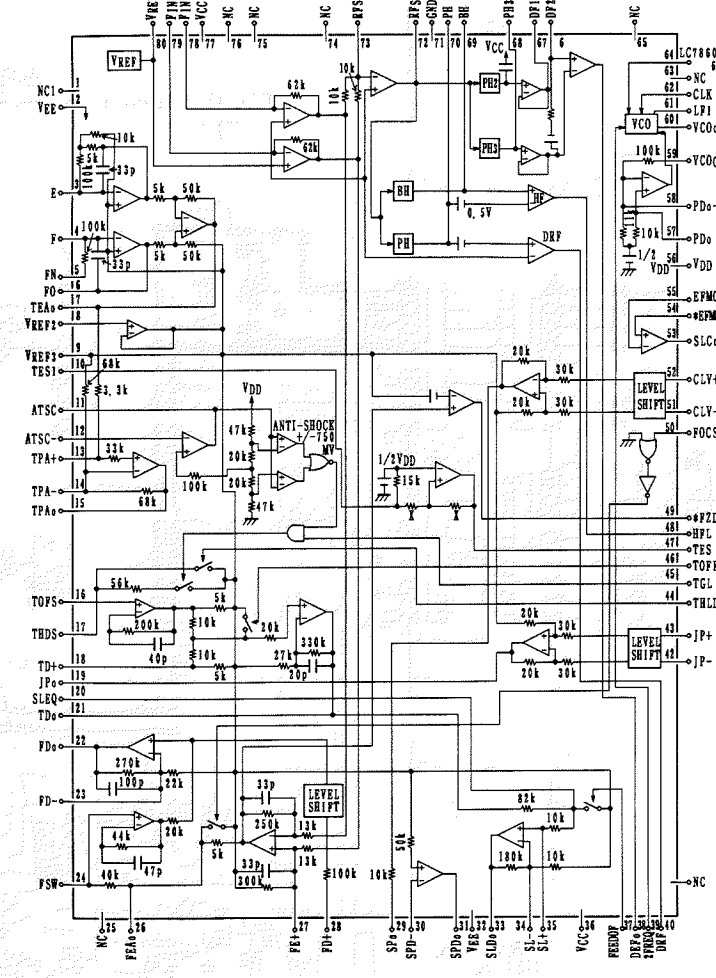
IC5 : LA9211M RF Amp & Servo Controller
