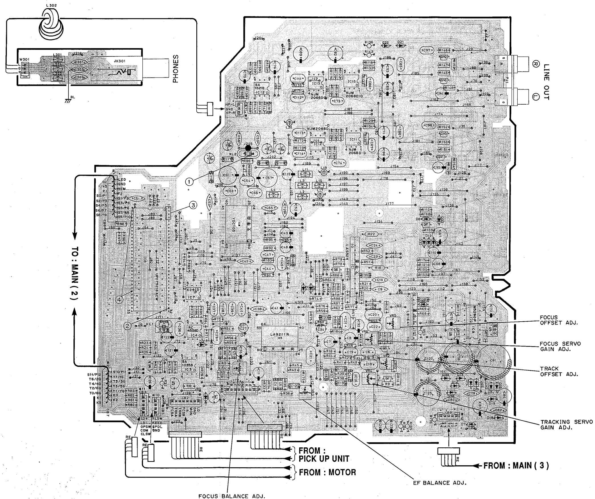
CDX - 470 MAIN P. C. B. ( 5 )
