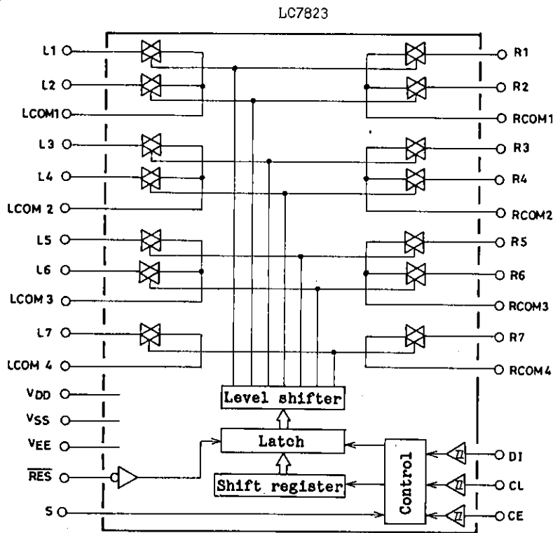
Equivalent Circuit Block Diagram
