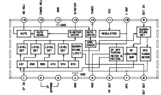
IC12 : LA1235
